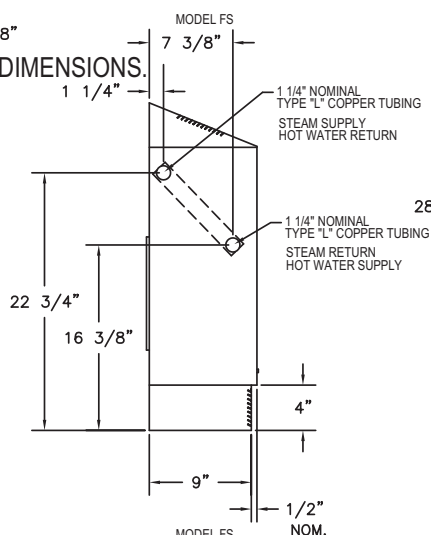
MODEL FS SIDE VIEW ARRANGEMENT FS-1005
