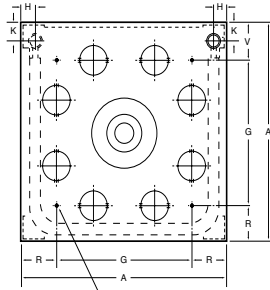
(4) MOUNTING HOLES 3/8" - 16 FOR MODELS 40-77
