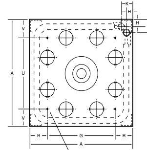
(4) MOUNTING HOLES 3/8" - 16 FOR MODELS 104-367 THREAD TAPS 1/2" - 13 FOR MODELS 495-700
