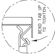
BOTTOM OF ACCESSORY INSTALLED AT ENCLOSURE BOTTOM
