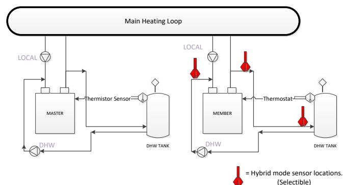
Simplified Drawing
