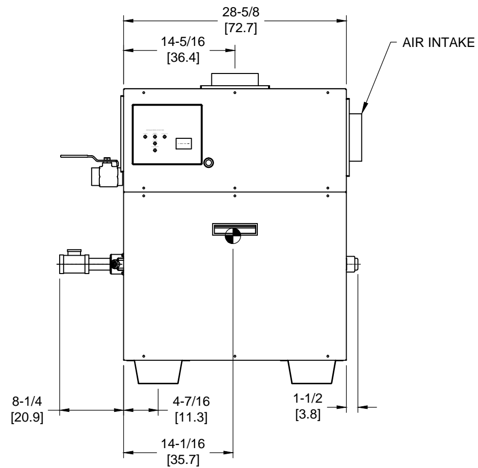
FRONT VIEW
