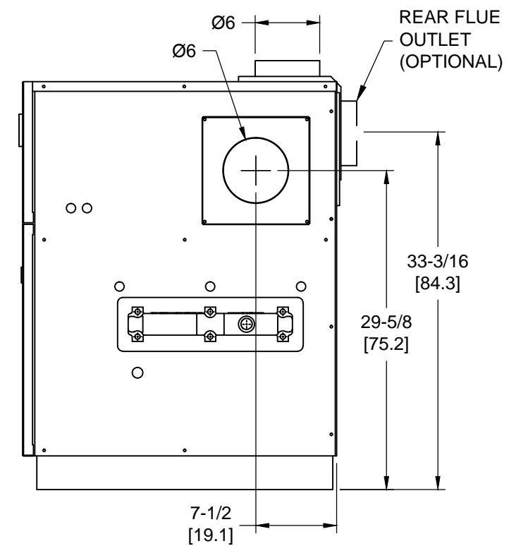
RIGHT VIEW
