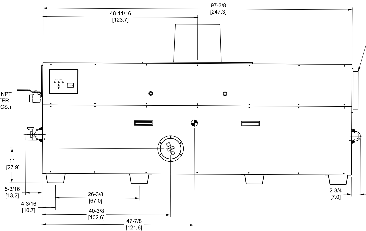
FRONT VIEW
