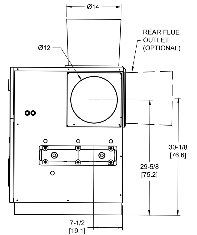
RIGHT VIEW
