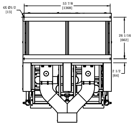
VIEW IN DIRECTION A BOTTOM VIEW
