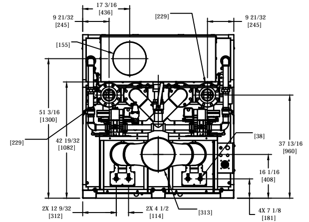
VIEW IN DIRECTION B ROTATED 180° CLOCKWISE BACK VIEW
