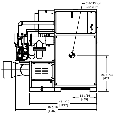
LEFT VIEW
