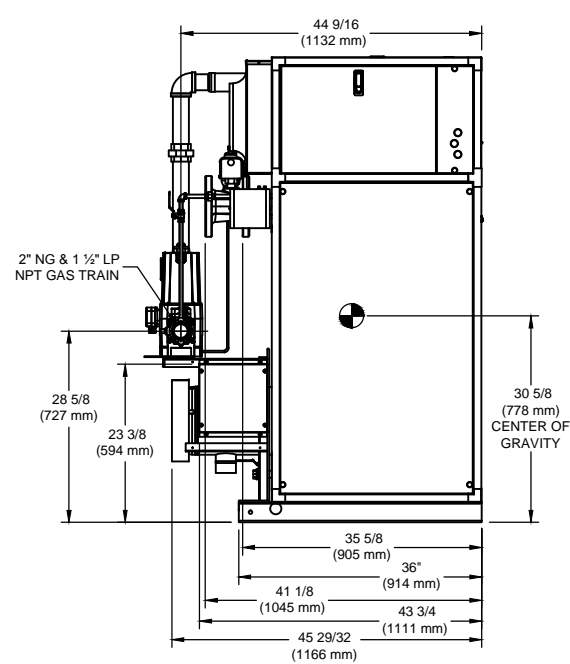
LEFT VIEW
