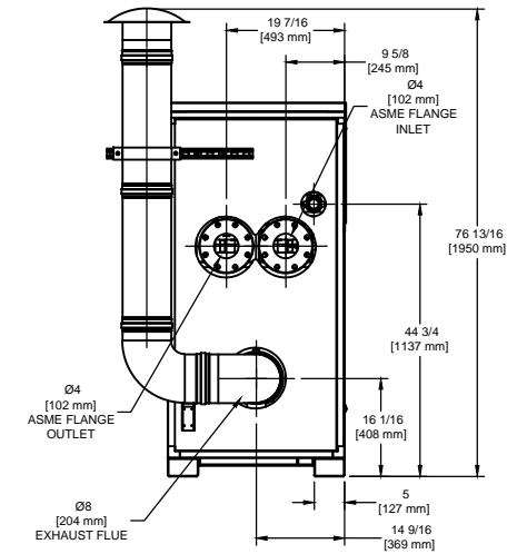
BACK VIEW
