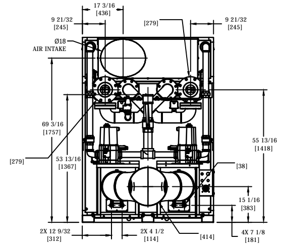
VIEW IN DIRECTION B ROTATED 180° CLOCKWISE BACK VIEW
