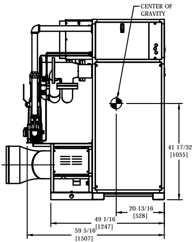
LEFT VIEW
