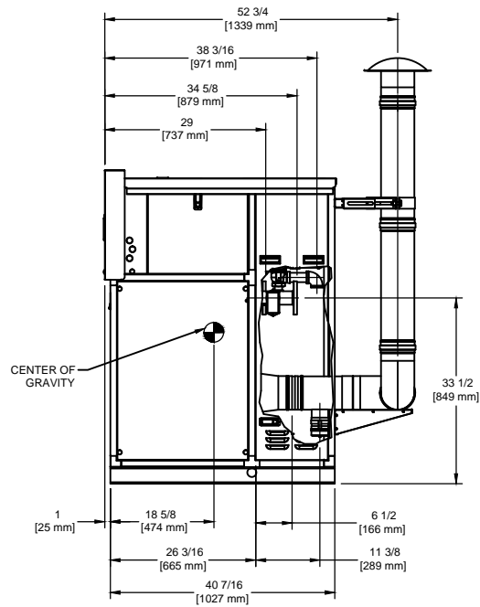
SIDE VIEW
