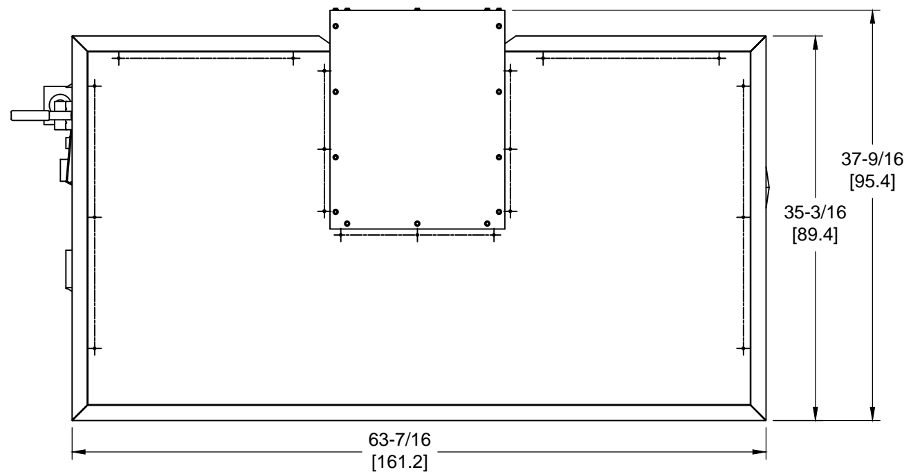
OUTDOOR TOP VIEW
