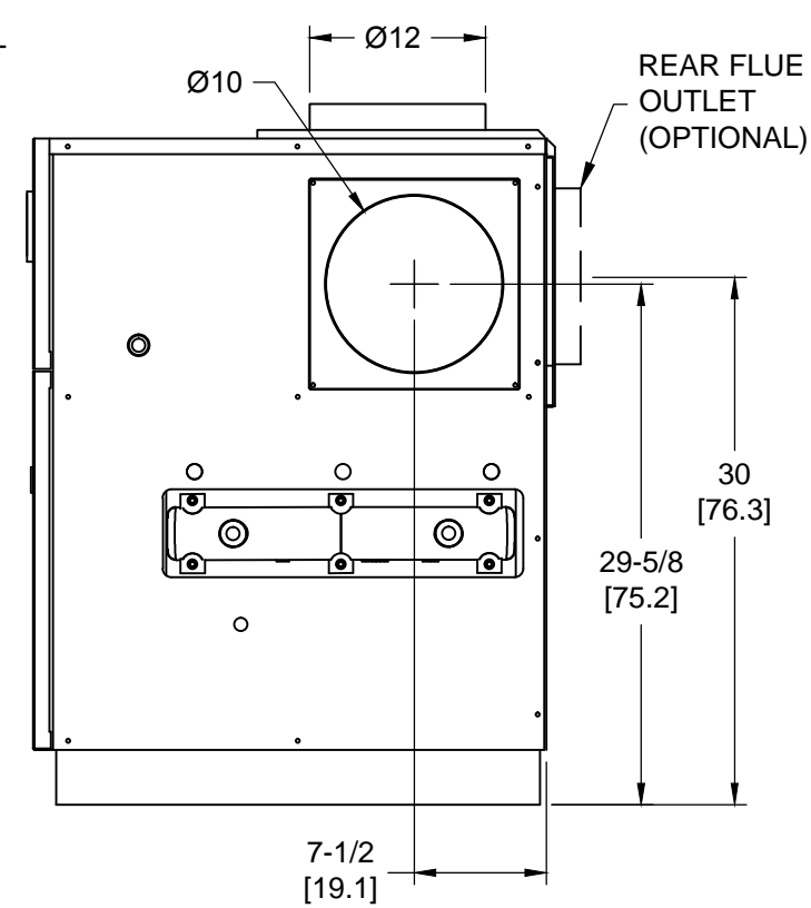
RIGHT VIEW
