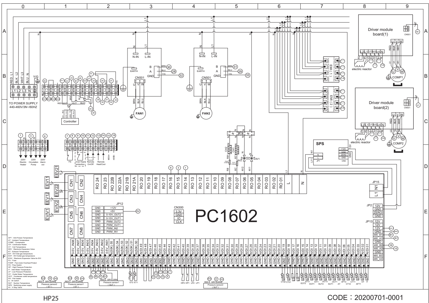
Figure 9 Wiring Diagram
