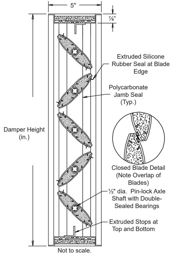
Opposed Blade Model shown (Parallel Blade Model also Available)
