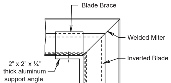
Mitered Corner Detail
