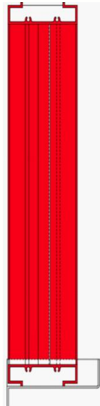
IL38 (3'') Vertical Chevron Storm Blade
