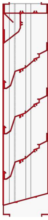
IL24 (4'') Double Drain
