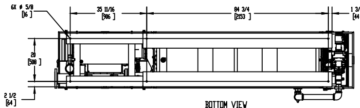
BOTTOM VIEW
