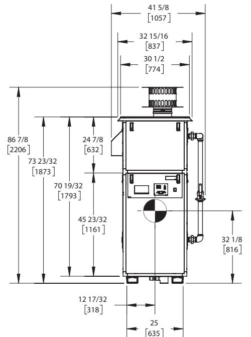
FRONT VIEW ASUB-00066_B
