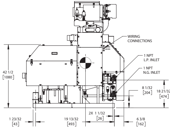
SIDE VIEW ASUB-00055_B
