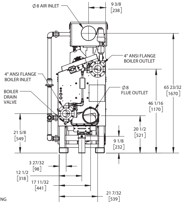
REAR VIEW ASUB-26_E
