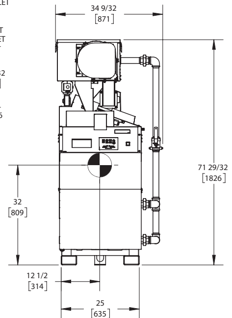
FRONT VIEW ASUB-26_E
