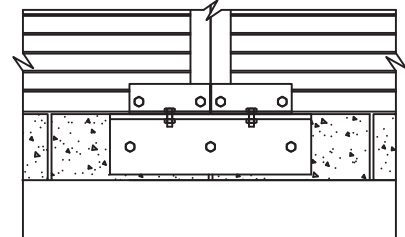
Model ALCF5 Recessed in Opening Head and Sill Detail
