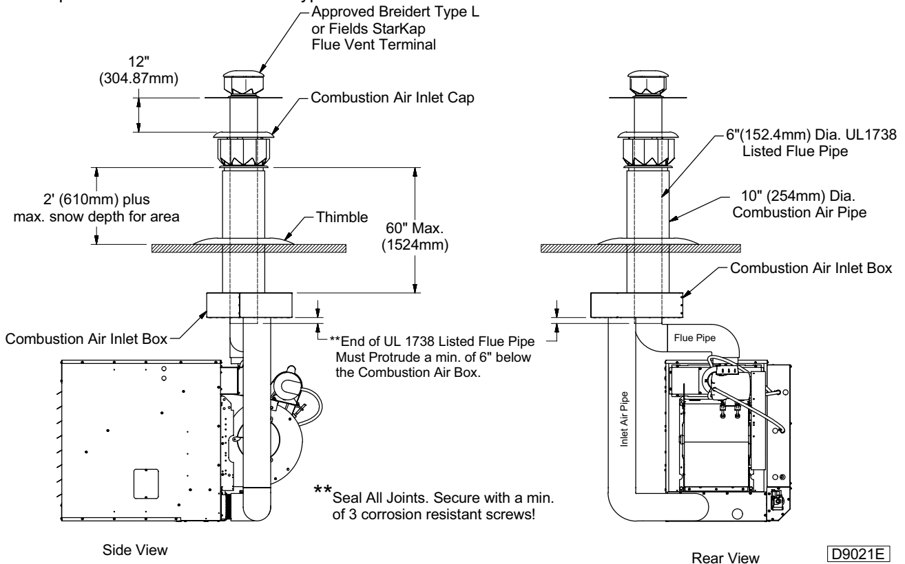
Figure 3b – Vertical 6 Inch Combustion Air Inlet Kit Installation
