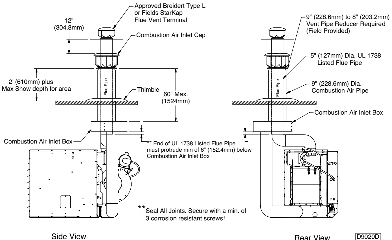
Figure 3a – Vertical 5 Inch Combustion Air Inlet Kit Installation
