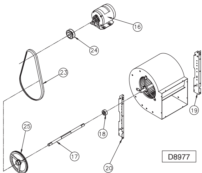
Figure 36 – Blower Assembly
