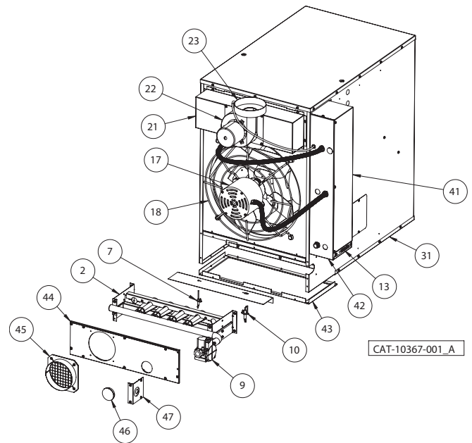
Figure 2 – Rear View
