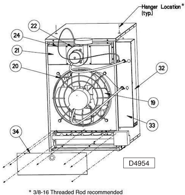
Figure 16 – Rear View
