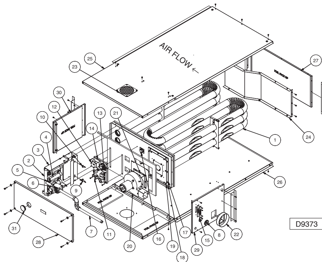
Figure 37 – Exploded View
