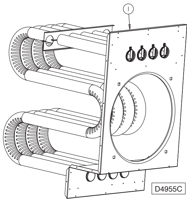
Figure 24 – Vestibule Panel/Tube Assembly (Heat Exchanger)
