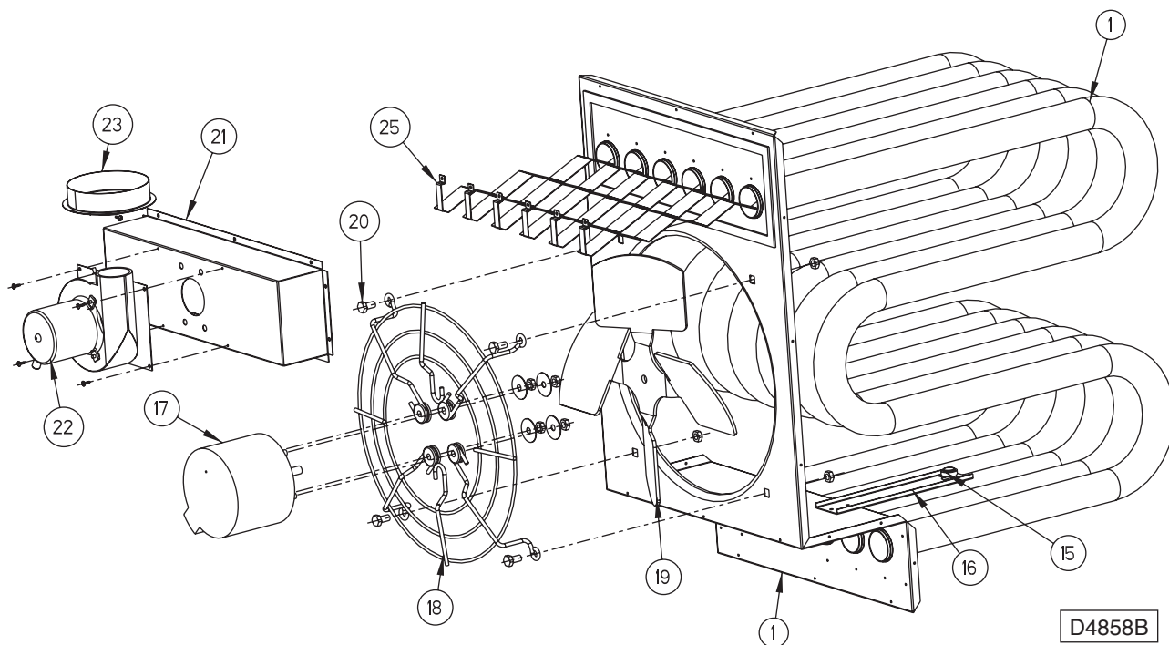
Figure 17 – Exploded View - Less Jacketry and Controls
