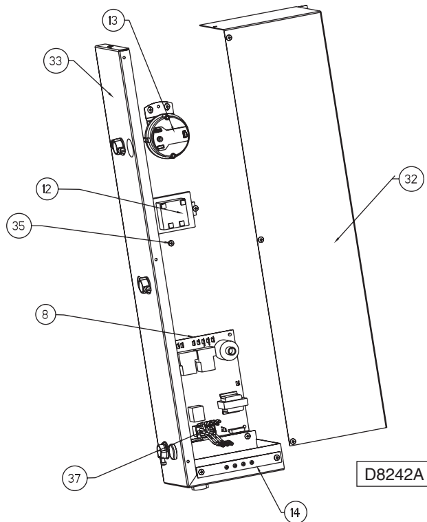
Figure 19 – Electrical Control Panel
