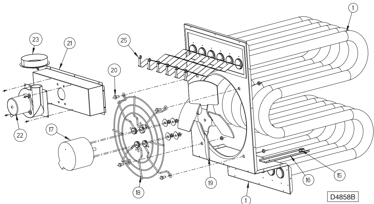
Figure 23 – Exploded View - Less Jacketry and Controls
