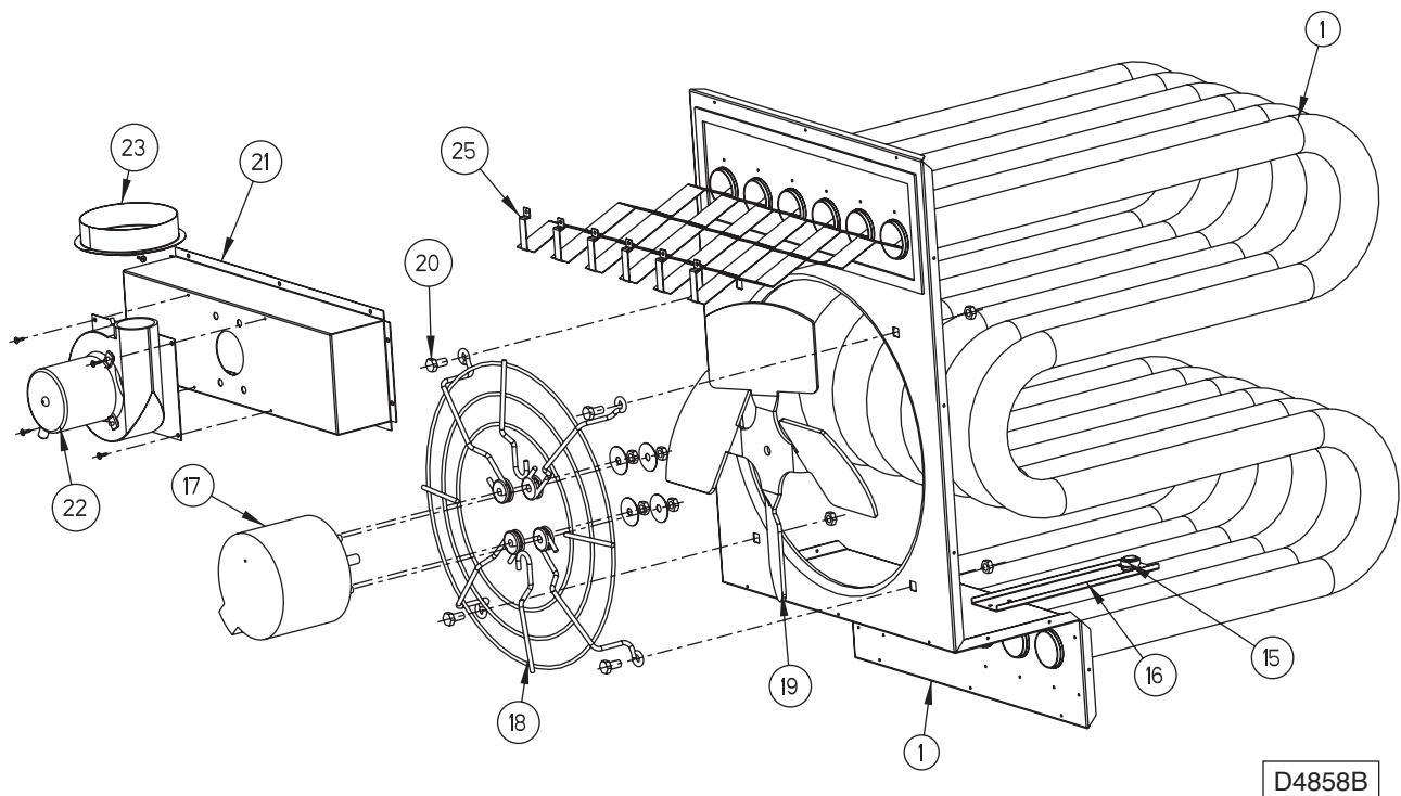
Figure 3 – Exploded View - Less Jacketry and Controls
