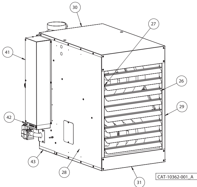
Figure 1 – Front View
