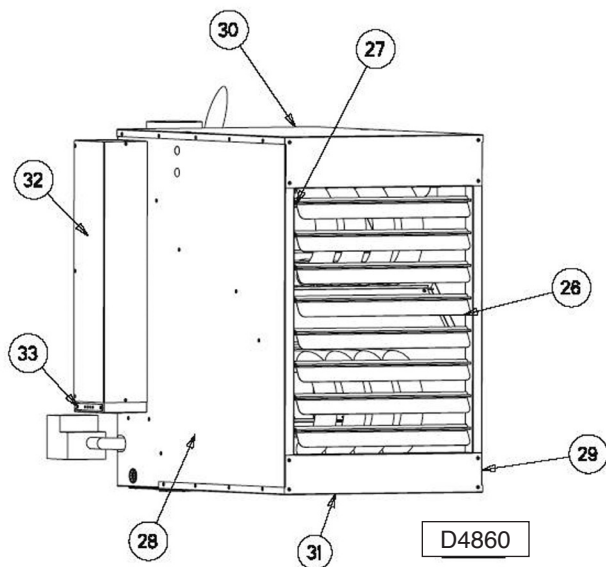
Figure 15 – Front View
