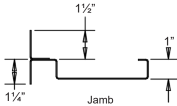
Flange Frame Available
