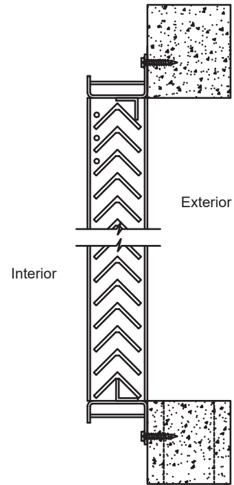
Model AL-UF5 Recessed in Opening Head and Sill Detail
