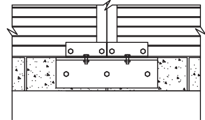
Model AL-UF5 Recessed in Opening Head and Sill Detail
