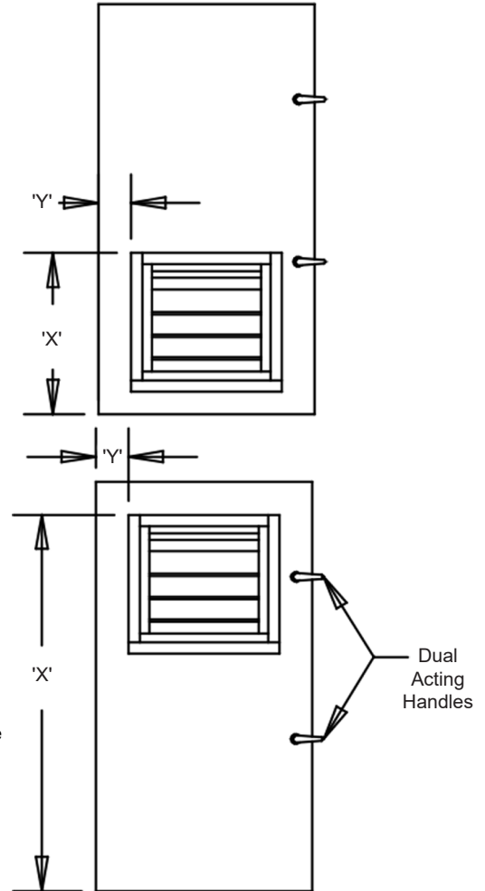
Door Panel View Minus Door Frame (Left hinge units shown.) Not to scale.
