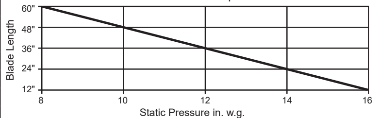
Model AFDTI-25LT Damper Limitations
