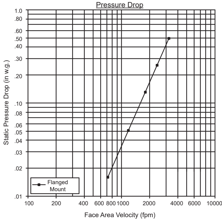
Model AFDTI-25LT Damper Size 36" x 36"
