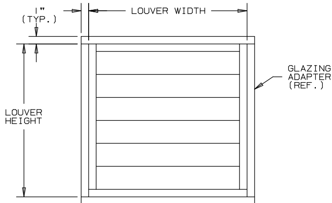
FRONT LOUVER ELEVATION
