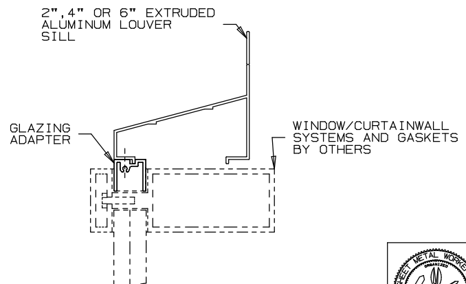
SILL DETAIL
