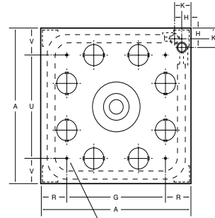
(4) MOUNTING HOLES \frac{3}{8} "-16 FOR MODELS 104-367D THREAD TAPS \frac{1}{2} "-13 FOR MODELS 495-700
