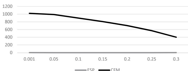
10 Ducted PSC CFM vs ESP @ High Speed
