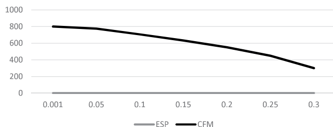
08 Ducted PSC CFM vs ESP @ High Speed
