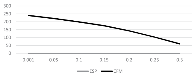
02 Ducted PSC CFM vs ESP @ High Speed
