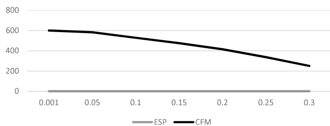
06 Ducted PSC CFM vs ESP @ High Speed
