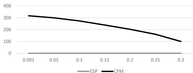
03 Ducted PSC CFM vs ESP @ High Speed
