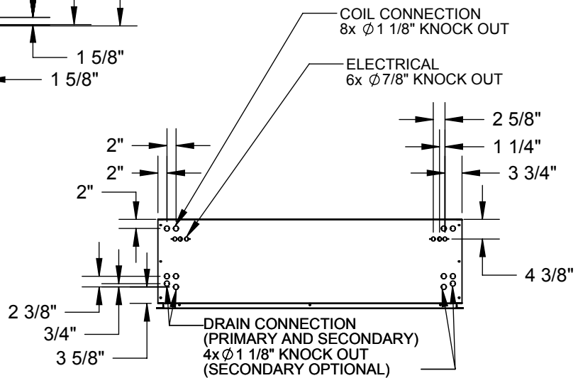
REAR VIEW (COIL CONNECTION)
