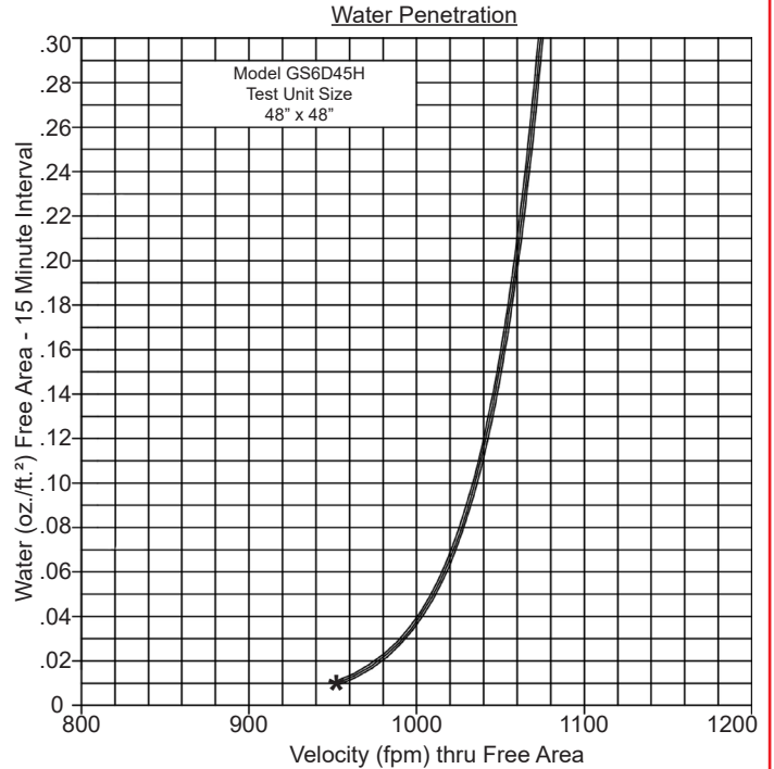
952 (FPM) Beginning Point of Water Penetration
