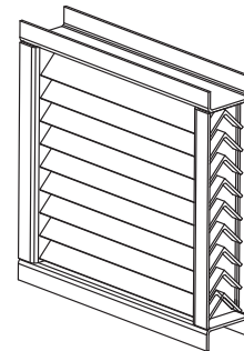
Optional Flange Mounting or Channel Frame Mounting
