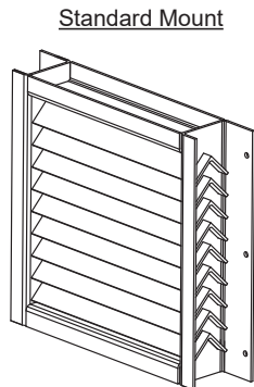
Cantilevered Mount Flange at Jambs
