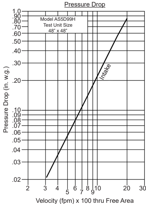
Velocity (fpm) x 100 thru Free Area Intake air converted to standard air density. Tested to AMCA Standard 500-L, Figure 5.5.
