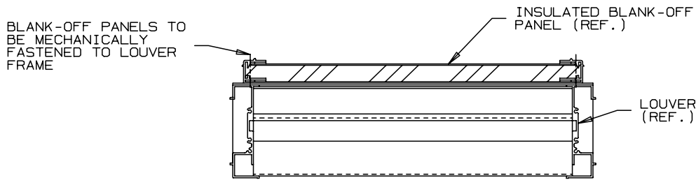
LOUVER ELEVATION
